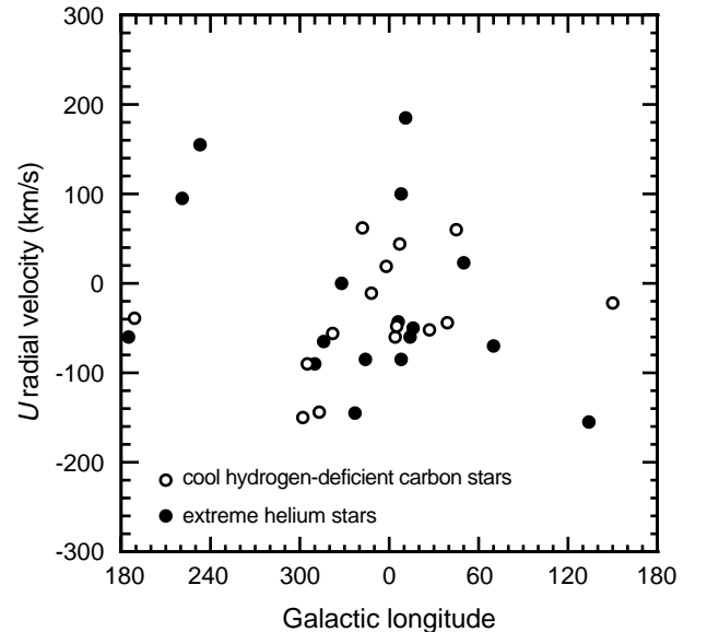
Figure 1 —The U radial velocity (positive towards the Galactic centre) versus Galactic longitude for cool hydrogen-deficient carbon stars (open circles) and extreme helium stars (filled circles; data from Drilling 1986). The velocity and spatial distribution of these types of stars is discussed in the text.
