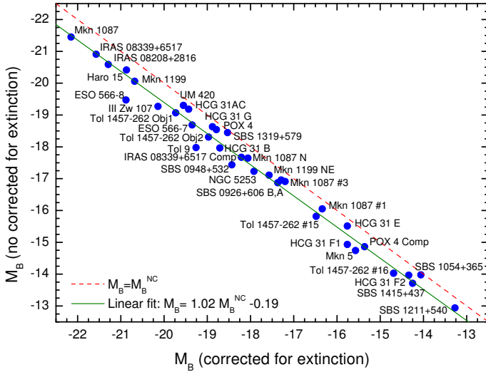
Fig. 1. Comparison between the reddening-corrected absolute B -magnitudes ( M_B ) and the uncorrected ones ( M_B^{NC} ) for all individual galaxies analysed in this work. A linear fit to the data is shown.
