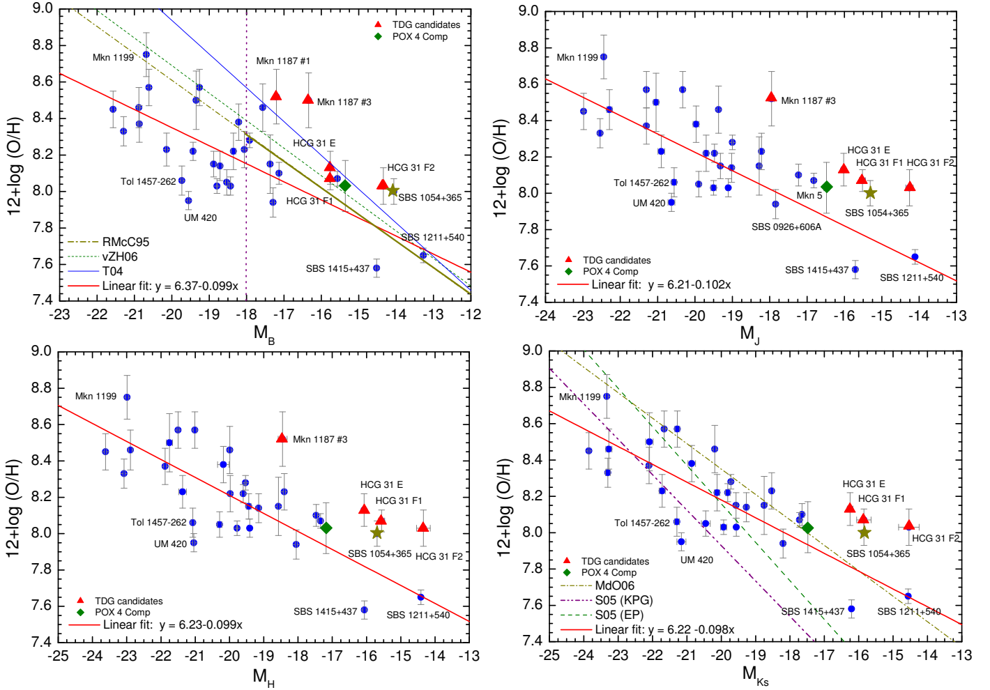
Fig. 17. Metallicity-luminosity diagrams for the objects analysed in this work. The oxygen abundance is expressed in units of 12+\log(O/H) ; the luminosity is expressed as the absolute magnitude in B , J , H and K_S filters. Red triangles represent the TDG candidates found in HCG 31 (López-Sánchez, Esteban & Rodríguez 2004a) and Mkn 1087 (López-Sánchez, Esteban & Rodríguez 2004b). A green diamond corresponds to the dwarf object surrounding POX 4, while a yellow star indicates the galaxy SBS 1054+365. Linear fits to our data are shown with a continuous red line in the four panels. The M_B -O/H diagram includes the relation derived by Richer & McCall (1995) (continuous dark yellow line) extrapolated to high luminosities (dashed-dotted dark yellow line), the relation provided by van Zee & Haynes (2006) (dashed green line), and the relation derived by Tremonti et al. (2004) using SDSS data (dotted blue line). The M_{K_S} -O/H diagram includes the two relations found by Salzer et al. (2005), one considering the Edmunds & Pagel (1984) calibration (EP, dashed green line) and another assuming the relationships provided by Kennicutt et al. (2003) (KPG, dashed-dotted purple line), and the relation found by Mendez de Oliveira et al. (2006) (dashed-dotted yellow line).
