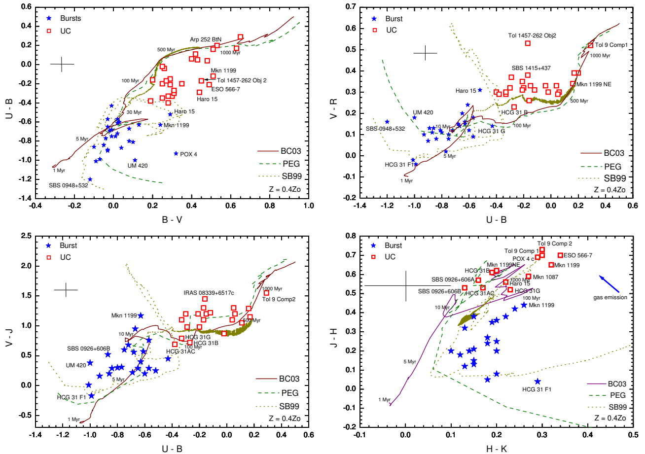
Fig. 2. Colour-colour diagrams comparing the predictions given by evolutionary synthesis models [continous line: BC03, Bruzual & Charlot (2003) models; discontinuous line: PEGASE.2, Fioc & Rocca-Volmerange (1997) models; dotted line: STARBURST 99, Leitherer et al. (1999) assuming Z = 0.4Z_{\odot} ] with the colours (corrected for both reddening and contribution of the emission lines) of our galaxy sample when the burst (blue stars) and underlying component (UC, red squares) of each system are considered independently. The cross indicates the typical errors in our data. Some age labels were included for the BC03 models.
