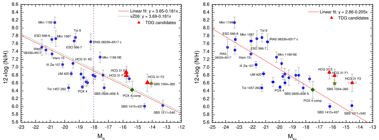
Fig. 18. Nitrogen abundance vs. luminosity for the galaxies analysed in this work. The nitrogen abundance is expressed in units of 12+\log(\text{N}/\text{H}) ; the luminosity is expressed as the absolute magnitude in B (left) and K_S (right) filters. Red triangles represent the TDG candidates found in HCG 31 (López-Sánchez, Esteban & Rodríguez 2004a) and Mkn 1087 (López-Sánchez, Esteban & Rodríguez 2004b). A green diamond corresponds to the dwarf object surrounding POX 4, while a yellow star indicates the galaxy SBS 1054+365. The relation derived van Zee & Haynes (2006) is plotted in the M_B -N/H relation with a green dashed line. The fits to our data are shown with a continuous red line.
