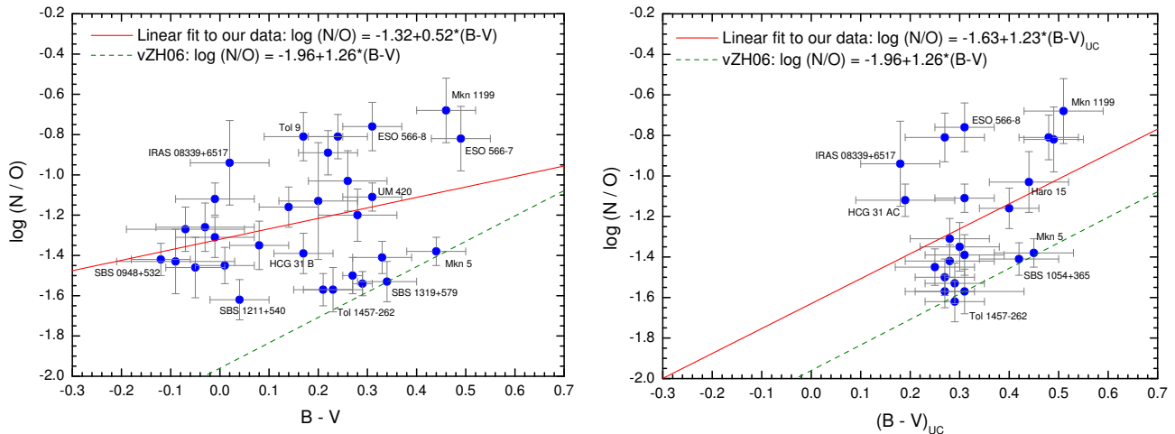
Fig. 20. N/O ratio vs. the reddening-corrected B-V colour considering all the galaxy (left) or just the underlying stellar population (right). A linear fit to our data is shown with a continuous red line. The relationship found by van Zee & Haynes (2006) in their analysis of dwarf irregular galaxies is plotted with a dashed green line.
