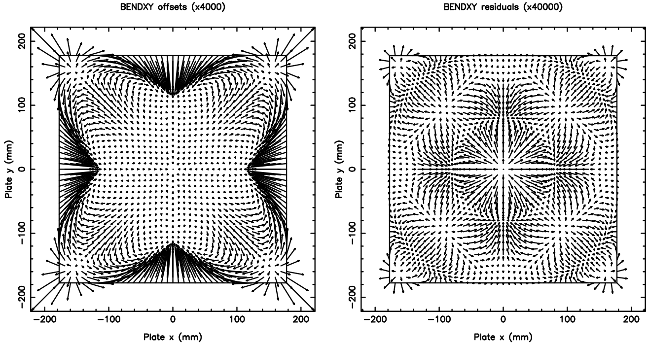
Fig. 3. (Left) Offsets ( \times 4,000 ) computed by BENDXY on a 40 \times 40 grid over the 350\text{mm} \times 350\text{mm} plate area. The rms deviation of the offsets is 3.7 \mu\text{m} and the maximum deviation is 15.4 \mu\text{m} . (Right) Residuals ( \times 40,000 ) of the BENDXY offsets after fitting by a 7th-degree polynomial in x , y , and r . The rms deviation of the residuals is 0.10 \mu\text{m} and the maximum deviation is 0.47 \mu\text{m} . Note that the residuals are scaled by an additional factor of \times 10 over the offsets.
