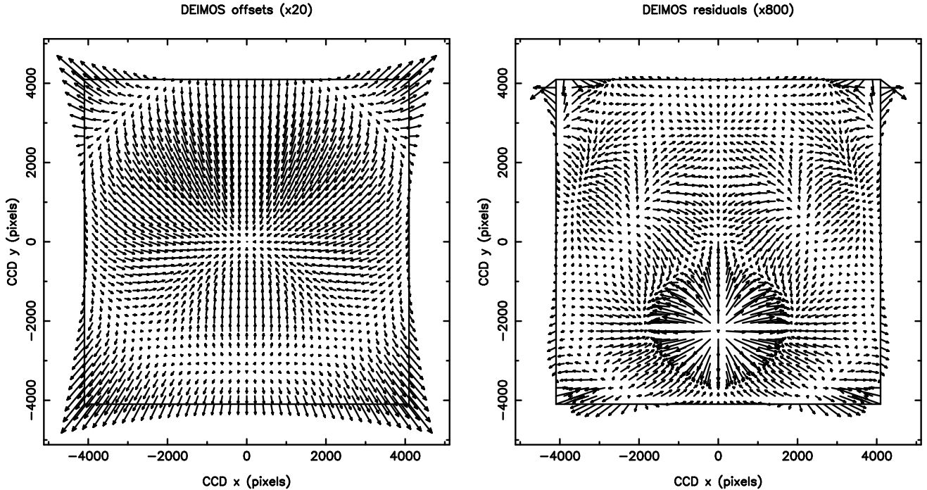
Fig. 4. (Left) DEIMOS offsets ( \times 20 ) computed on a 40 \times 40 grid over the 8192 \times 8192 pixel CCD array. The rms deviation of the offsets is 7.3 pixel with maximum deviation 46.3 pixel. (Right) Residuals ( \times 800 ) of the DEIMOS offsets after fitting by a 7th-degree polynomial in x , y , and r . The residuals, which are scaled by an additional factor of \times 40 over the offsets, have an rms deviation of 0.19 pixel and a maximum deviation 1.38 pixel. This corresponds to 23 and 164 milliarcsec at the stated scale of 0.119 arcsec/pixel.
