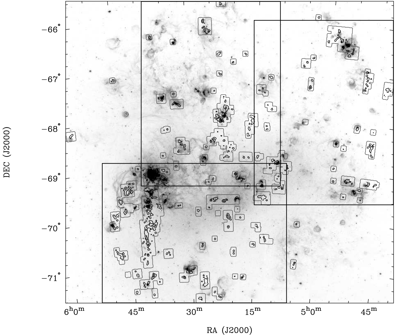
Figure 1. CO intensity contours from MAGMA, at levels of 2 and 10 K km s -1 , overlaid on an H \alpha image from MCELS (Smith et al. 1999), shown on a logarithmic stretch to bring out fainter emission. The CO image was derived by smoothing the MAGMA cube to 1' resolution and applying a blanking mask corresponding to the 3 \sigma contour of a 1.5'-resolution smoothed cube. Multiple small rectangular contours show the regions mapped in CO with Mopra. Large rectangular boxes show the regions magnified in Figures 5 and 6. The H \alpha image has not been continuum subtracted, although bright point sources have been removed by a moving boxcar median filter.
