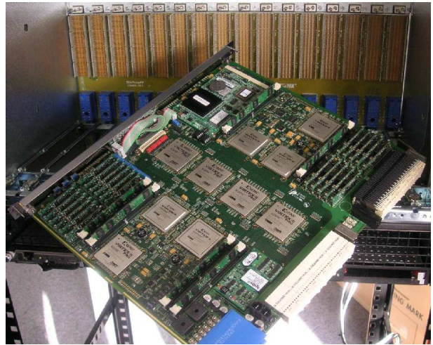
Figure 8. The CABB Digital Signal Processing (DSP) board.
