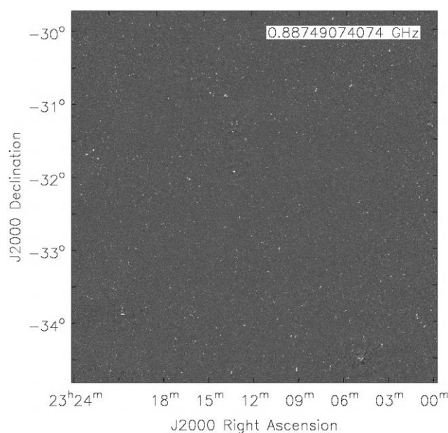
Main region of the first GAMA23 field with an intensity scale covering 99.5% of the total range.
