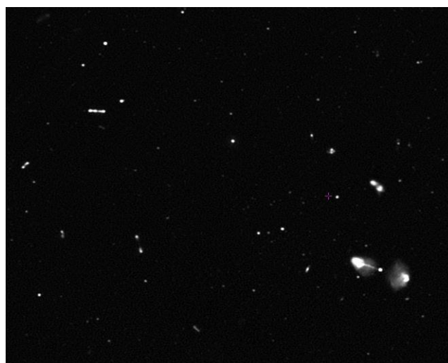
Close-up of the second tile, showing a giant radio galaxy in the bottom-right and many others scattered throughout the field.
