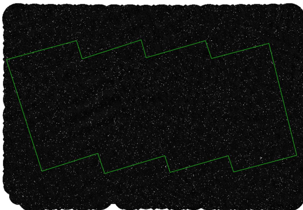
Preliminary mosaicked image of the 888 MHz SWAG-X continuum data, with eROSITA eFEDS coverage marked in green
