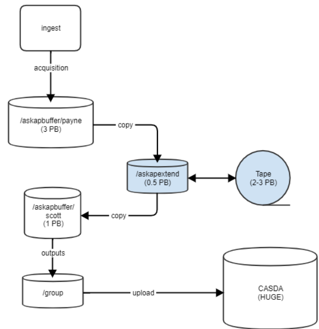
ASKAP data flow diagram highlighting the new tape stage
