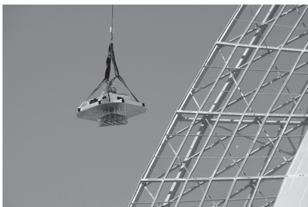
Installation of a 300 – 900-MHz receiver on the Parkes 64-m radio telescope. The wideband feed is based on the Eleven Feed, designed by Per-Simon Kildal of Chalmers University, Sweden.
