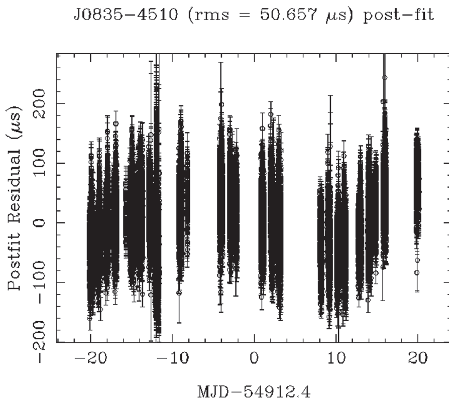
Figure 1: Vela timing residuals from observations with the ASKAP 12-m test-bed antenna. The data sets will be made available on the PULSE@Parkes websites with a range of on-line projects that will let the students interact with the data. We hope that our small project will allow us to develop remote observing capabilities, obtain useful scientific data and provide a new aspect of the PULSE@Parkes project. We also are considering further educational/scientific projects that could be undertaken with the 12-m antenna, such as getting students to observe the HI line and would be interested in any other suggestions.
