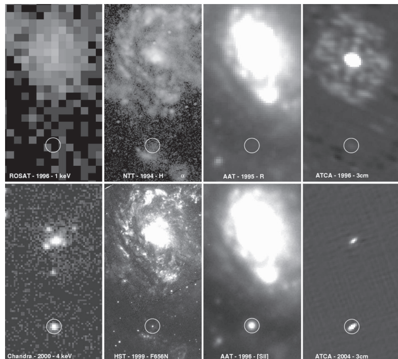
Figure 1: Observations of SN1996cr and its host galaxy at X-ray (left column), optical (middle columns), and radio wavelengths (right column) shortly before or around the time of the SN explosion (upper panel) and several years after the explosion (lower row).
