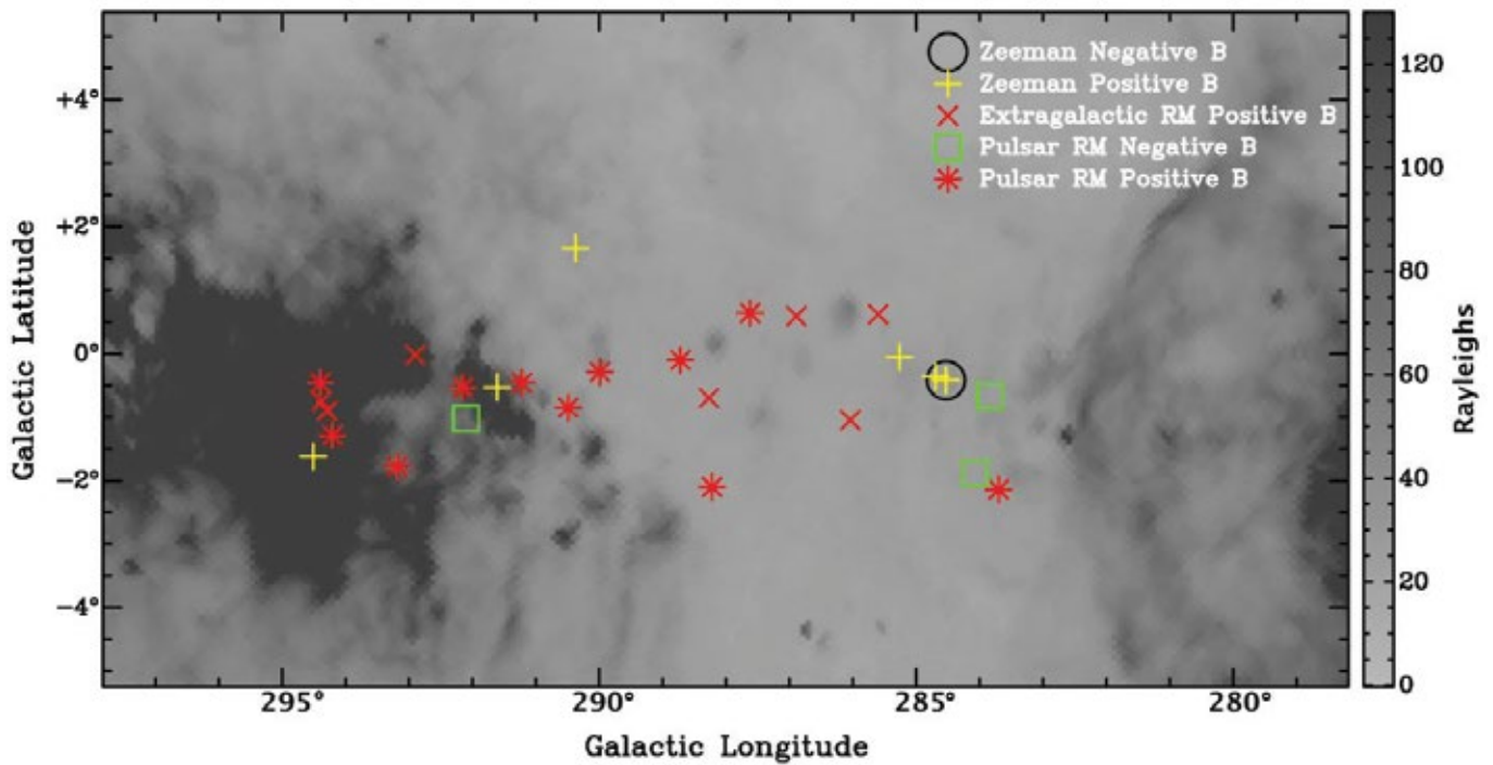
FIGURE 2: This figure (from Green et al. 2012) compares the magnetic field directions from rotation measures and Zeeman splitting measurements, overlaid on the composite H-alpha emission of Finkbeiner (2003) using the Southern H-Alpha Sky Survey Atlas data of Gaustad et al. (2001). The H-alpha emission indicates regions of ionised hydrogen. Yellow pluses are positive magnetic field Zeeman measurements (conventionally fields away from us) and a black circle is the sole site of negative magnetic field Zeeman measurements (a field towards us); red asterisks are positive rotation measures (fields towards us) from pulsars; green squares are negative rotation measures (fields away from us) from pulsars (Taylor et al. 1993; Han et al. 1999, 2006) and red crosses are positive rotation measures (fields towards us) from extragalactic sources (Brown et al. 2007). The rotation measures, from both pulsars and extragalactic sources, are all along lines of sight in the proximity of, or directly passing through, HII regions (Nota and Katgert 2010, references therein).
