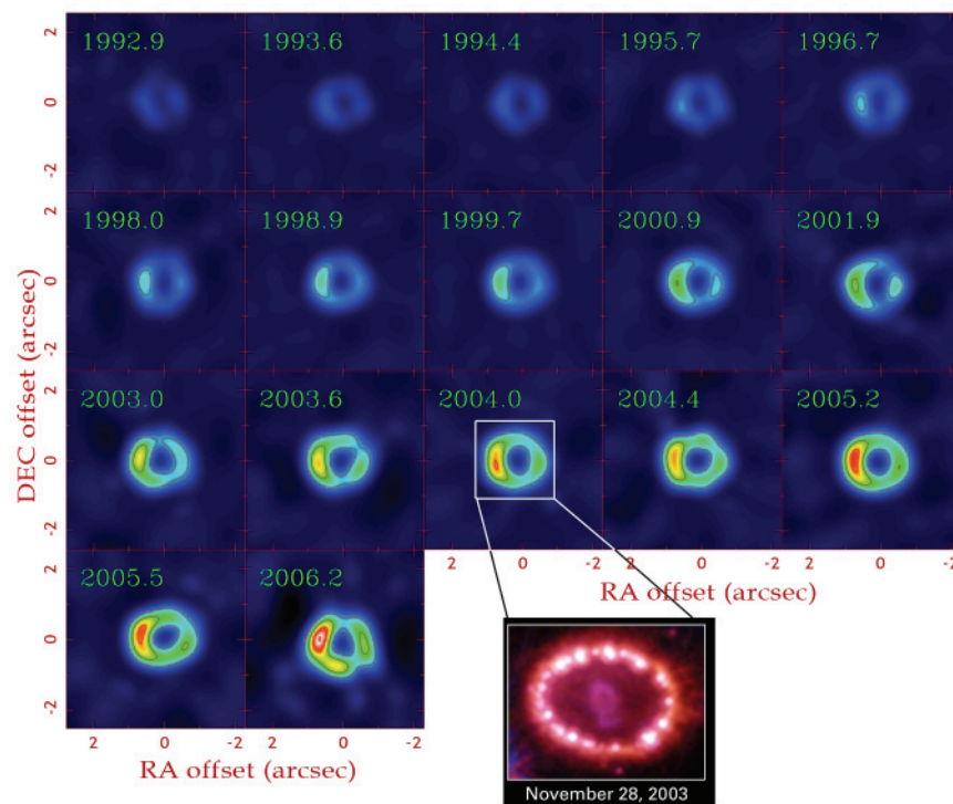
Compact Array observations of SN1987A at 8 GHz between 1992 and 2006. The images shown have been super-resolved to a resolution of 0.5 arcsec and were taken at multiple frequencies in the 3-cm band and typically include two complementary 6-km configurations. The inset photo is a high-resolution optical image from the Hubble Space Telescope's Advanced Camera for Surveys (ACS), courtesy NASA, P. Challis, R. Kirshner and B. Sugerma.
