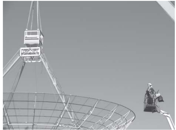
The THEA tile being mounted on the eastern New Technology Demonstrator antenna.
