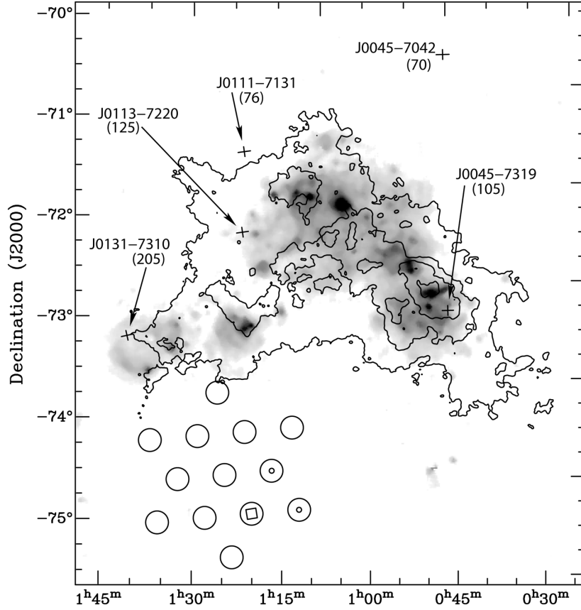
Figure 2: Multi-wavelength image of the field surrounding the burst. The grey scale and contours respectively show H \alpha and H I emission associated with the Small Magellanic Cloud. Crosses mark the positions of the five known radio pulsars in the Small Magellanic Cloud. Open circles show the positions of the 13 beams in the original survey pointing, with squares showing the beams in which we detected the burst.
