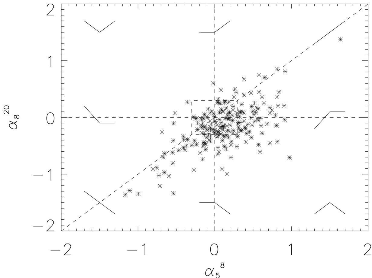
Figure 2: Colour-colour radio plot for the 218 sources with 20-GHz flux densities of > 0.5 Jy with near-simultaneous observations at 20, 8 and 5 GHz.
