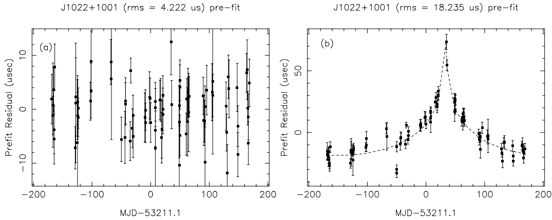
Figure 7. The timing residuals, in \mu\text{s} , for PSR J1022+1001, (a) after fitting for the pulsar’s parameters and (b) without removal of the Solar system Shapiro delay. This plot was created using the PLK plug-in for TEMPO2 (note, the original PLK plotting package incorrectly plotted the uncertainties on the residuals; the errors were a factor of 2 too small).
