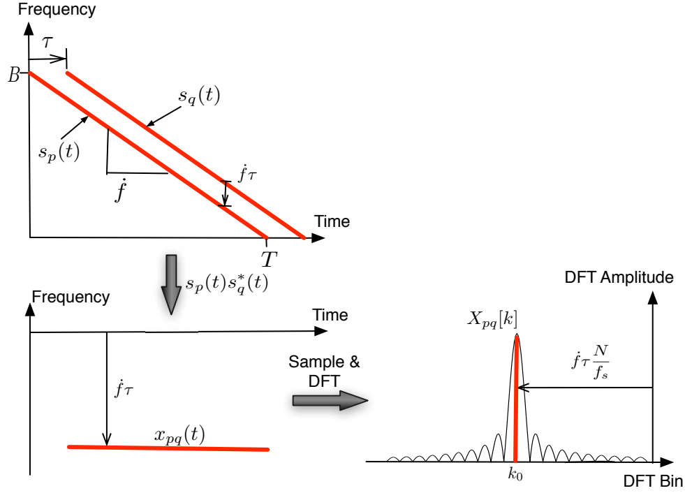
Figure 4.3: Schematic illustrating the “the Chirpolator” operating with two antennas. Top left: two linear chirps are received by antennas p and q , with one delayed by \tau . Bottom left: after taking the product of the two voltage time series, the result x_{pq} has constant frequency over most of the duration of the chirp. Bottom right: the DFT of x_{pq} yields a peak at k_0 .
