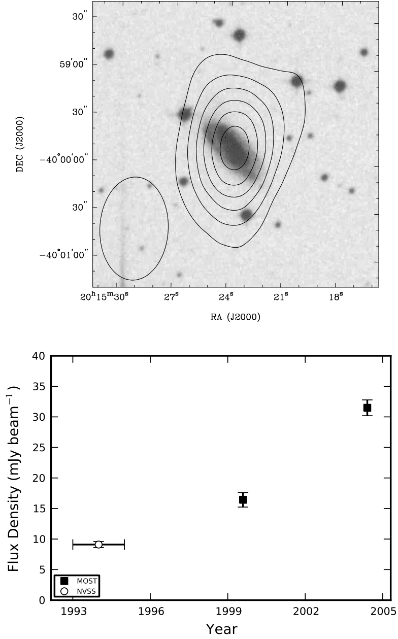
Figure 2.24: Variable radio source J201524–395949. Top panel: MOST contours from 5 to 30 mJy beam -1 in steps of 5 mJy beam -1 for the brightest epoch (2004 May 1) overlaid on a SuperCOSMOS B image. Bottom panel: light curve showing an NVSS detection and a doubling in 843 MHz flux density over 5 years over a 6 year interval.
