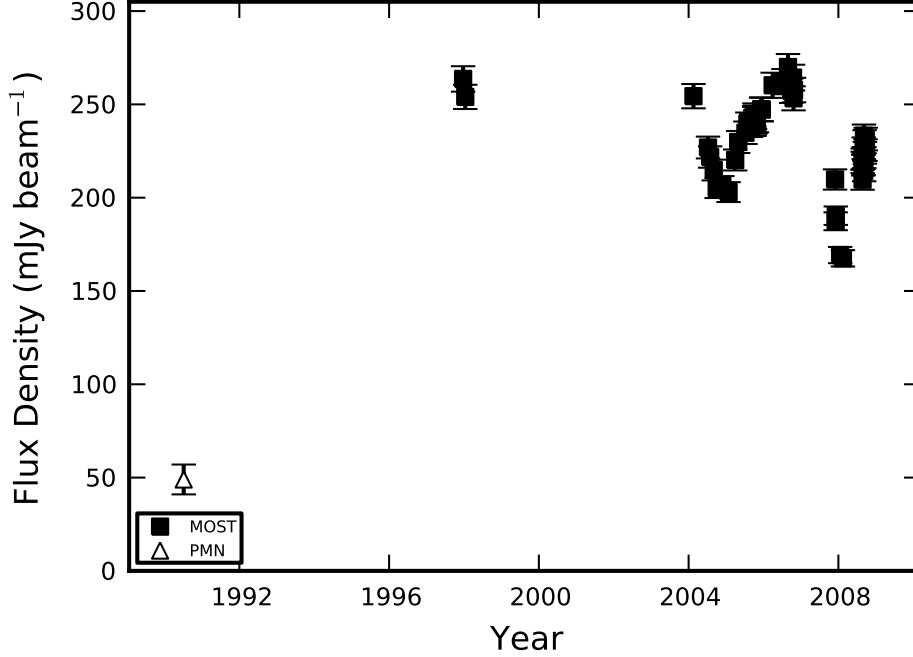
Figure 2.26: Light curve of the candidate compact steep spectrum source: SUMSS J223255–615308
