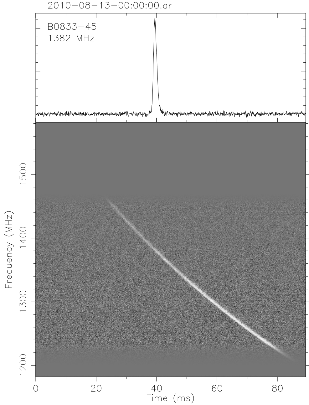
Figure 1.5: Dispersion by the ISM causes frequency a dependent delay. Plotted above is the folded radio pulse from the Vela pulsar (PSR B0833-45) which has a period of 89 ms and a DM of 67.99 \text{ pc cm}^{-3} . These data were recorded in 60 s with the 12 m telescope used to take the measurements in Chapter 3. Top panel: dedispersed time series showing shape of the pulse emitted by the pulsar, before being dispersed by the ISM. Bottom panel: frequency vs. time image where the gray scale is the intensity of the incoming radiation. The \nu^{-2} dispersion sweep is seen between 1220 and 1460 MHz. The telescope feed has no sensitivity outside these frequencies.
