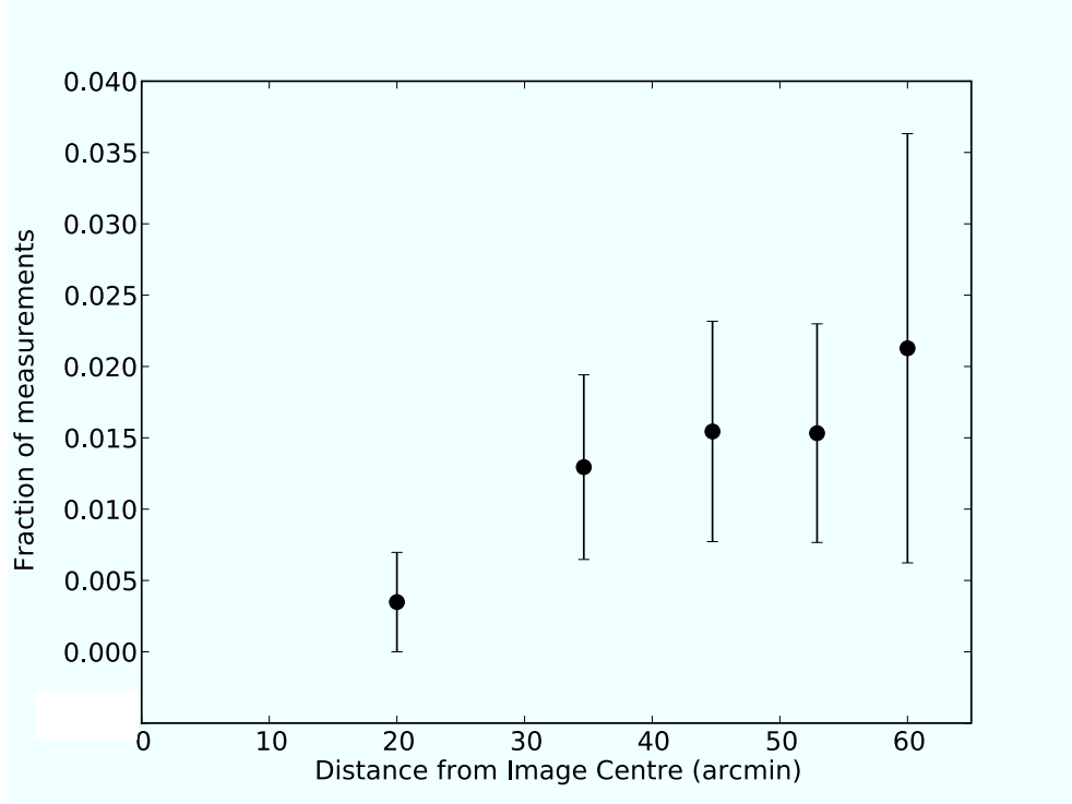
Figure 2.15: Plot of the fraction of flux density measurements that deviate from \bar{S} by more than 20 per cent, binned by distance from the image centre. Only images centred on the HDFs were considered, and 2 known variable sources were removed. The error bars are Poisson errors
