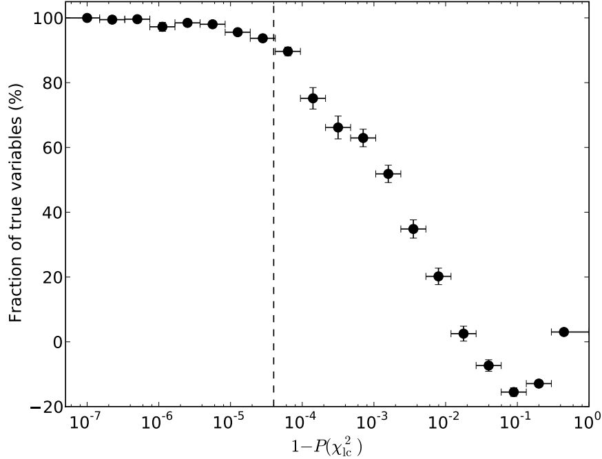
Figure 2.14: Confidence measure, C(T) vs 1 - P(\chi^2_{lc}) on a log scale. To achieve a fraction of genuine variable sources of 90 per cent requires 1 - P(\chi^2_{lc}) = 4 \times 10^{-5} . The y errors are the Poisson errors propagated through the definition of the confidence metric, and the x errors indicate the bin width. The confidence is negative at large values of 1 - P(\chi^2_{lc}) due to a deficiency of moderately variable sources at large values of 1 - P(\chi^2_{lc}) (see Fig. 2.13.). The dashed vertical line indicates the adopted threshold of 1 - P(\chi^2_{lc}) = 4 \times 10^{-5} = T_0 , to the left of which the confidence of finding a genuinely variable source is greater than 90 per cent.
