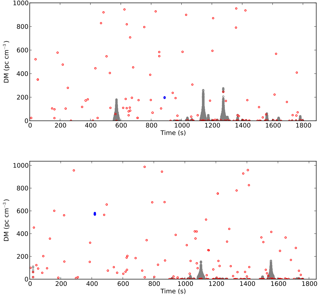
Figure 3.1: DM vs. time for the two GRBs with single-pulse candidates. Single-pulse detections with a significance \geq 6\sigma appear as circles in this plot, with the size proportional to the S/N. The detections are colour coded according to their classification by the friends-of-friends algorithm as candidates (blue), false positives (red) and RFI (grey). Top panel: GRB 100704A with a single pulse candidate 1076 seconds after the GRB at a DM of 195 \text{ pc cm}^{-3} , with a significance of 6.2\sigma and width of 6 ms. Bottom panel: GRB 101011A with a single pulse candidate 524 seconds after the GRB at a DM of 570 \text{ pc cm}^{-3} , with a significance of 6.6\sigma and width of 25 ms. The time origin of these plots is the time that the telescope first arrived on source ( T_{\text{on}} ).
