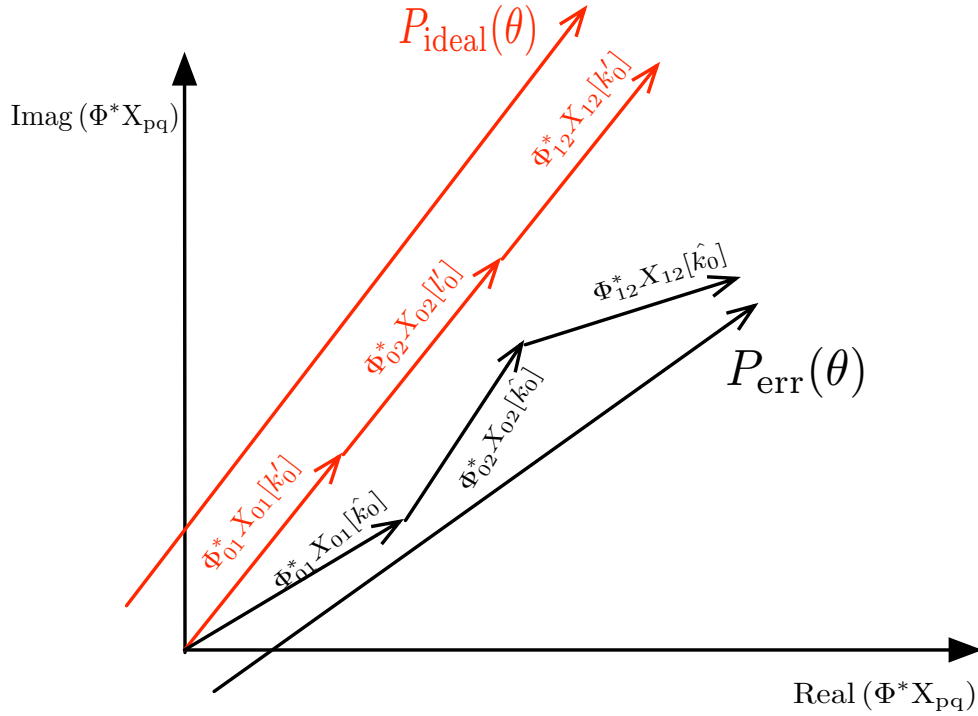
Figure 4.7: Errors in delay calibration reduce the amplitude of the detection metric. Here we plot the formation of the detection metric P(\theta) as the vector (i.e., complex) sum of the phase-corrected DFT results from three antenna pairs. In the ideal case (red), the phase correction ( \Phi_{pq}^* ) perfectly corrects for the known phase in the DFT bins ( X_{pq} ), and each result has the same absolute phase. The resulting detection metric ( P_{\text{ideal}}(\theta) ) is fully coherent. If delay errors are present, each DFT bin has a residual phase that is different for each antenna pair. The resulting detection metric ( P_{\text{err}}(\theta) ) has a smaller amplitude, because the vectors do not add into a straight line.
