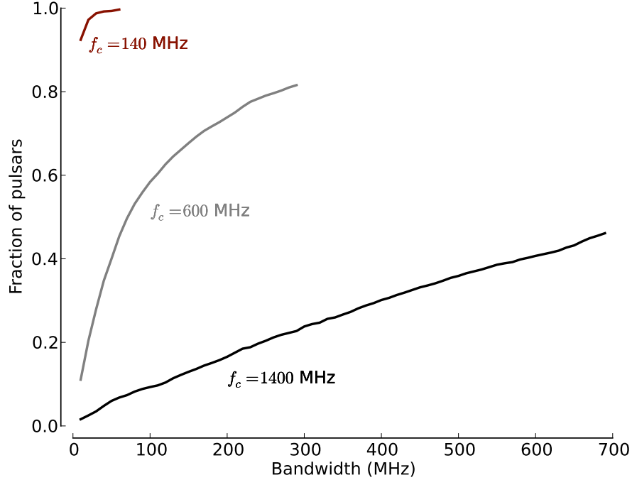
Figure 4.8: Fraction of known pulsars that violate the isolated chirp condition, as a function of system bandwidth and centre frequency ( f_c ). Known pulsars are taken from the ATNF pulsar catalogue.
