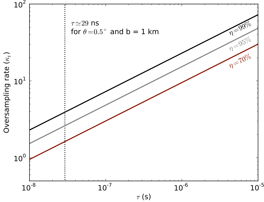
Figure C.3: One method for handling nonlinear dispersion with the Chirpulator is to increase the oversampling rate. Above is the required oversampling rate ( \kappa_t ) for a nonlinear chirp vs. the geometric delay ( \tau ) for single a baseline operating at f_c = 1.4 GHz, B = 400 MHz, and a range of different coherence losses ( \eta ). The vertical dashed line is the geometric delay for \theta = 0.5^\circ and a baseline of 1 km. The required oversampling rate is independent of DM.
