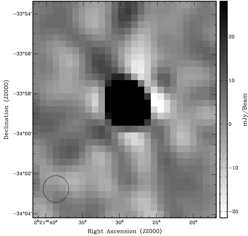
Figure 2.6: Example of poor dirty beam modelling producing negative regions around SUMSS J022129–335825 after CLEANing. Fitting a 2D Gaussian in a 10 \times 10 \text{ pixel}^2 region centred on the source results in an integrated flux density of 394.0 mJy which is less than peak intensity of 449.3 \pm 16.6 \text{ mJy} . The size of the fitted Gaussian is consistent with the size of the synthesised beam (shown in the bottom left). The large difference in integrated and peak flux densities is due to poor dirty beam modelling.
