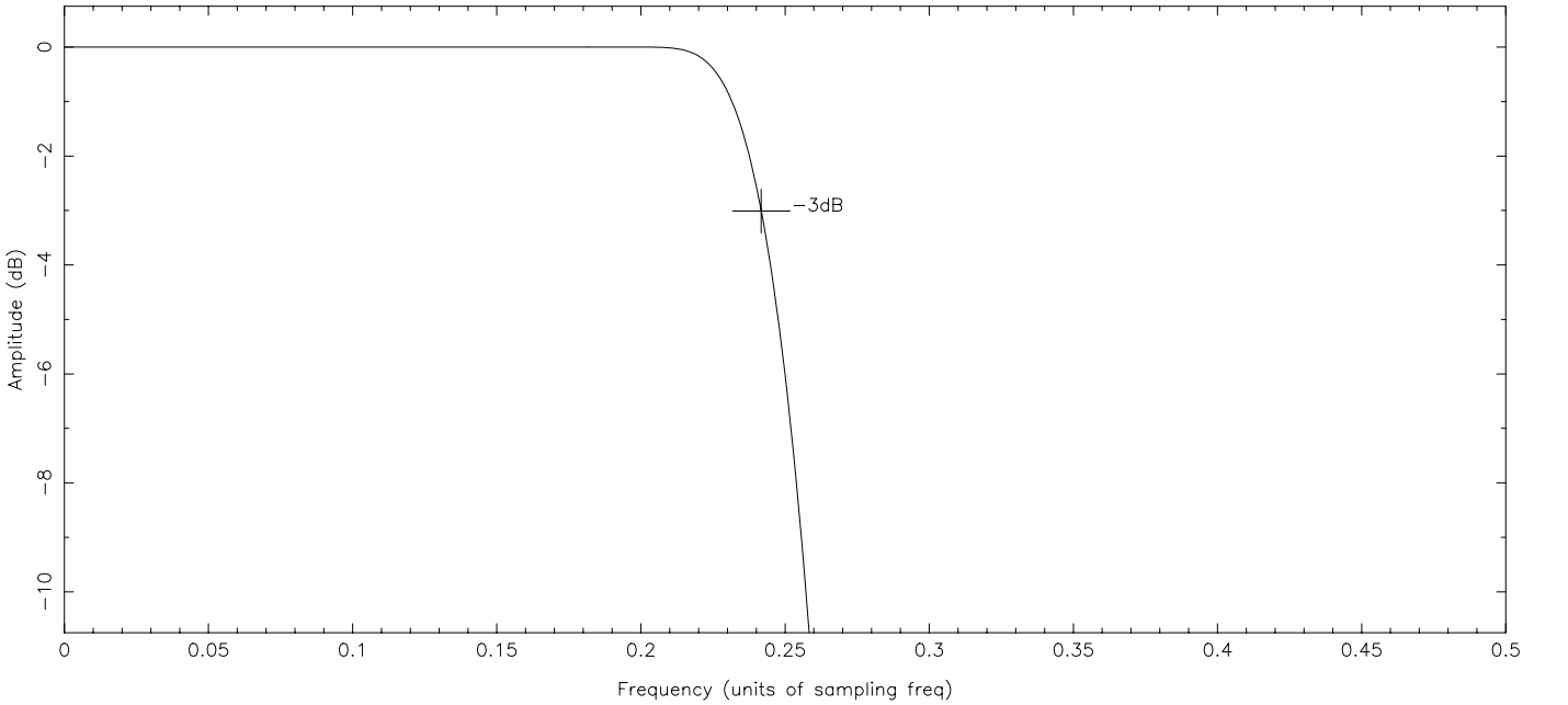
FIR Frequency Response – Expanded Scale
